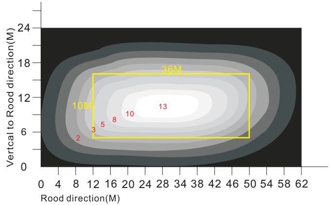
Lamp height:12M The effective lumination area can be realized just as the yellow rectangular area indicated ,36M*10M. Average lumination: 9Lux. Road surface evenness ratio:68%
