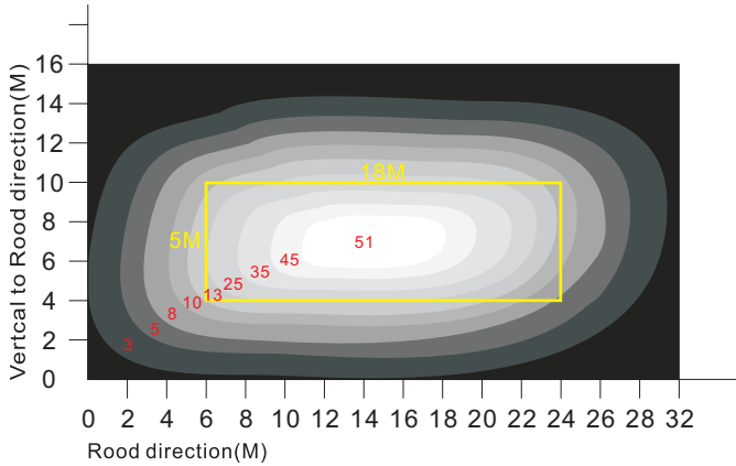
Lamp height:6M The effective lumination area can be realized just as the yellow rectangular area indicated ,18M*5M. Average lumination: 39Lux. Road surface evenness ratio:68%
