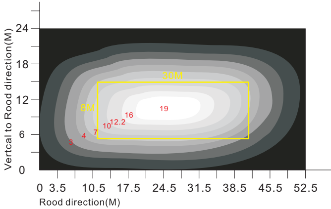
Lamp height:10M The effective lumination area can be realized just as the yellow rectangular area indicated ,30M*8M. Average lumination: 14Lux. Road surface evenness ratio:68%
